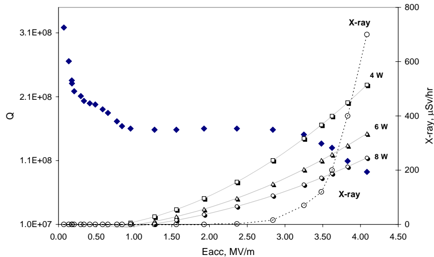
Figure 3. Q vs. E_a curves of the best ANU SLR re-plated using the Slotolet MSA process
