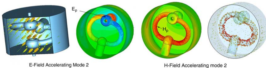
Figure 1. Low frequency accelerating mode for distributions of E-Field and H-field in SLR.
