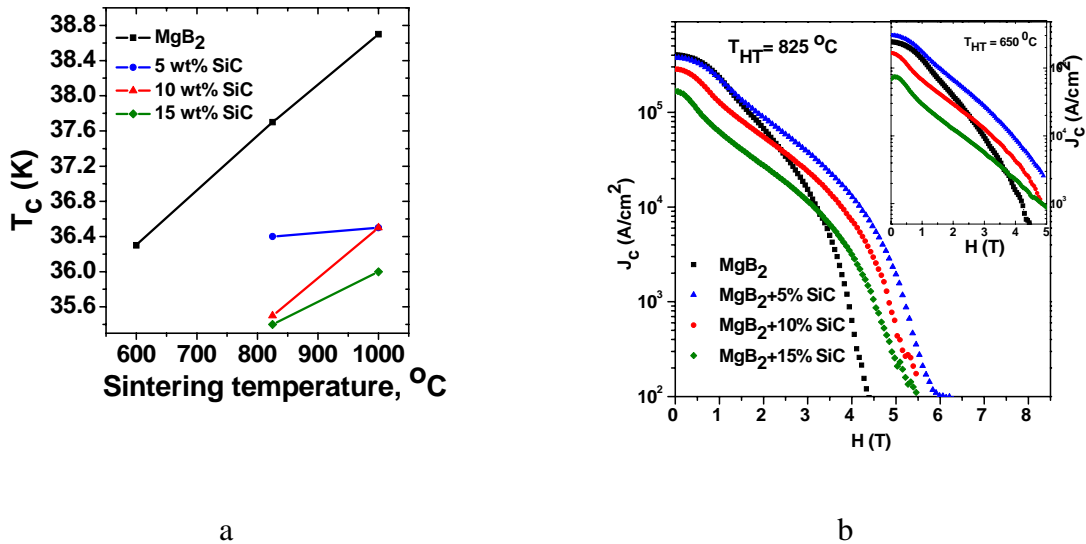
Figure 1. a) Critical temperature of studied samples vs sintering temperature; b) critical current density of pure and SiC added MgB 2 samples sintered at 825 0 C and 650 0 C (insert).
