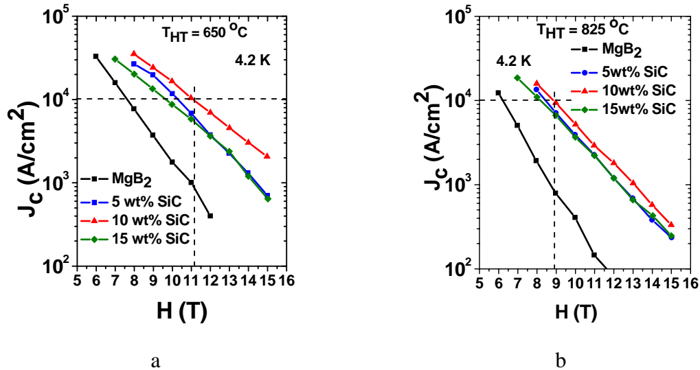
Fig. 2. Transport critical current densities of samples sintered at 650 o C (a) and 825 o C (b).
